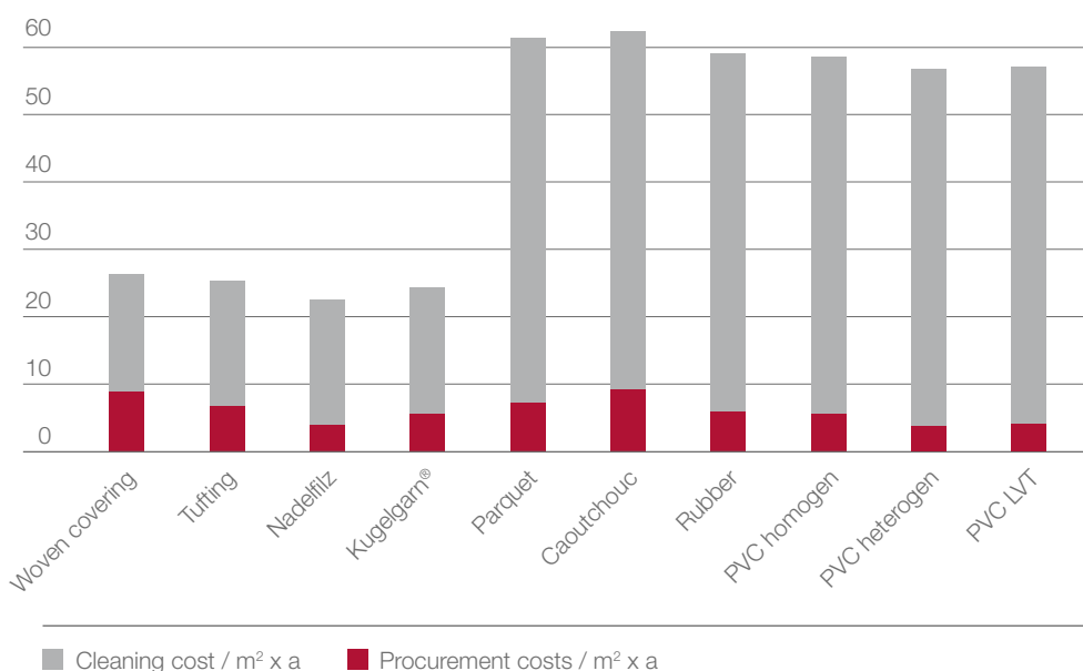
Annual costs for different types of floor covering (CHF pro m 2 x a)
