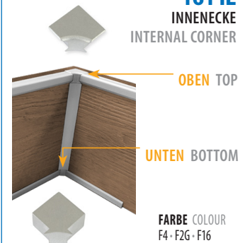
2-TEILIGE CLIP-INNENECKE 2-PART CLIP INTERIOR CORNER
