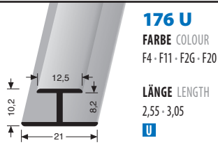
H-VERBINDER H CONNECTOR
