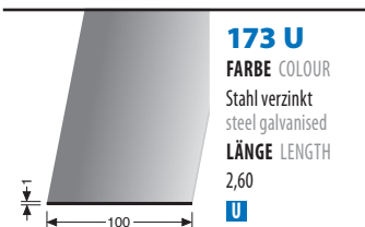
PLATTENSTOSS-SCHIENE PANEL JOINT RAIL
