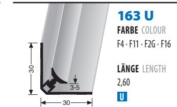
2-TEILIGE CLIP-INNENECKE 2-PART CLIP INTERIOR CORNER
